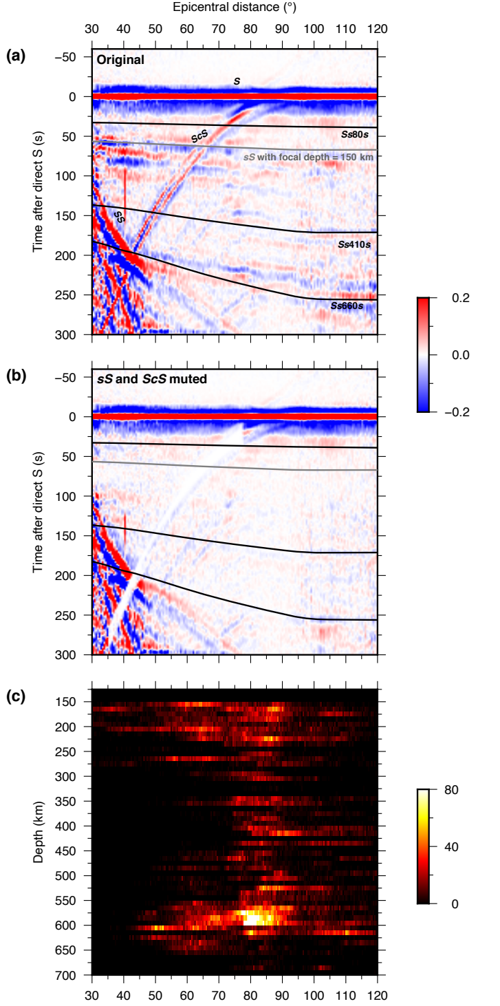
Figure 4. (a) Record section of traces included in our analysis. Note the strong depth phases that overprint reflections deeper than 150 km. The black and gray curves mark the predicted arrival times for reflections at 80, 410, 660 km depth, and sS for a focal depth of 150 km, respectively. Also note the interference of ScS . (b) The same as (a) but with sS and ScS muted using their predicted arrival times. Note that the 410 and 660 reflections start to emerge after the interfering sS phases are muted. (c) Distribution of event depth and distance.
