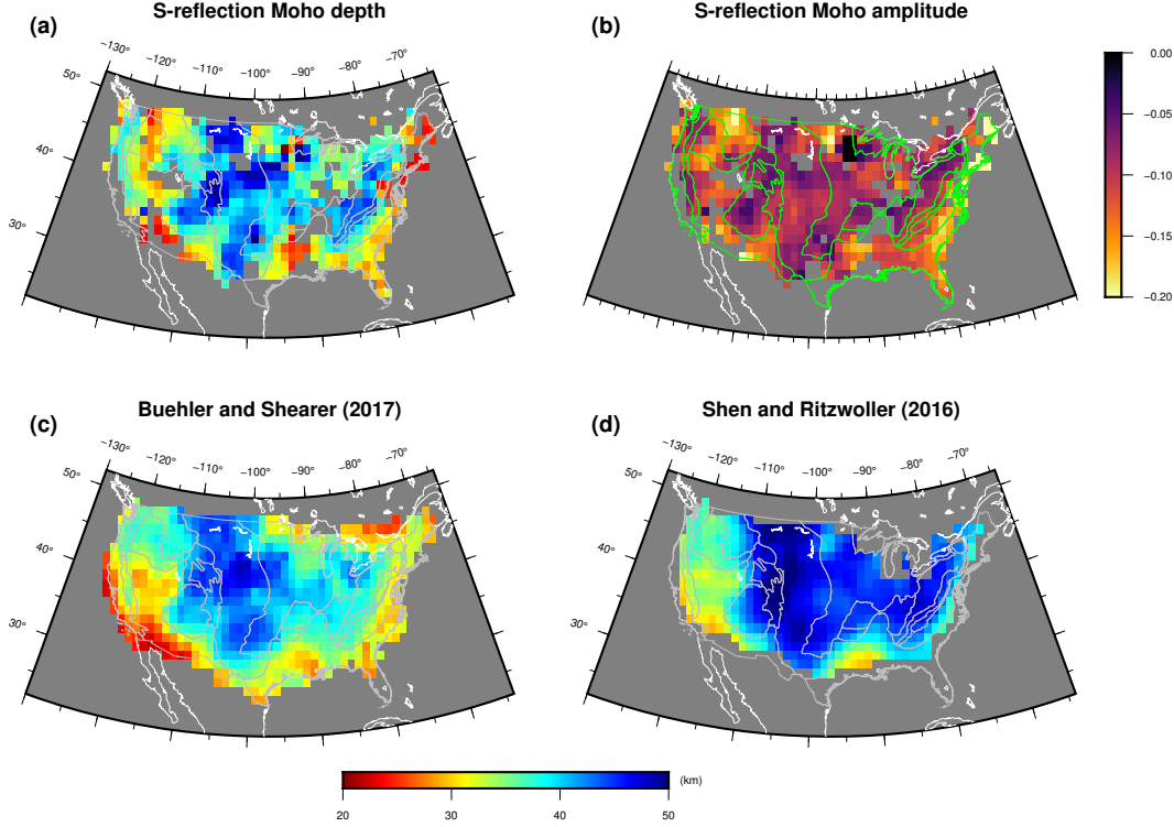
Figure 7. Comparison between our Moho observations and previous studies. (a) and (b) Moho depth and amplitude, respectively, from our S-reflection CRP image volume. (c) Moho depth from Buehler and Shearer (2017). (d) Moho depth from Shen and Ritzwoller (2016).
