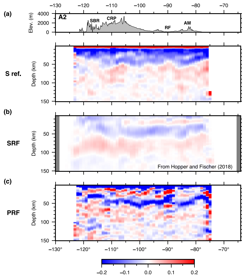
Figure 6. Comparison between (a) our S-reflection image, (b) SRF image from Hopper and Fischer (2018), and (c) our PRF image for Profile A2. Acronyms for key tectonic features are the same as in Figure 5.
